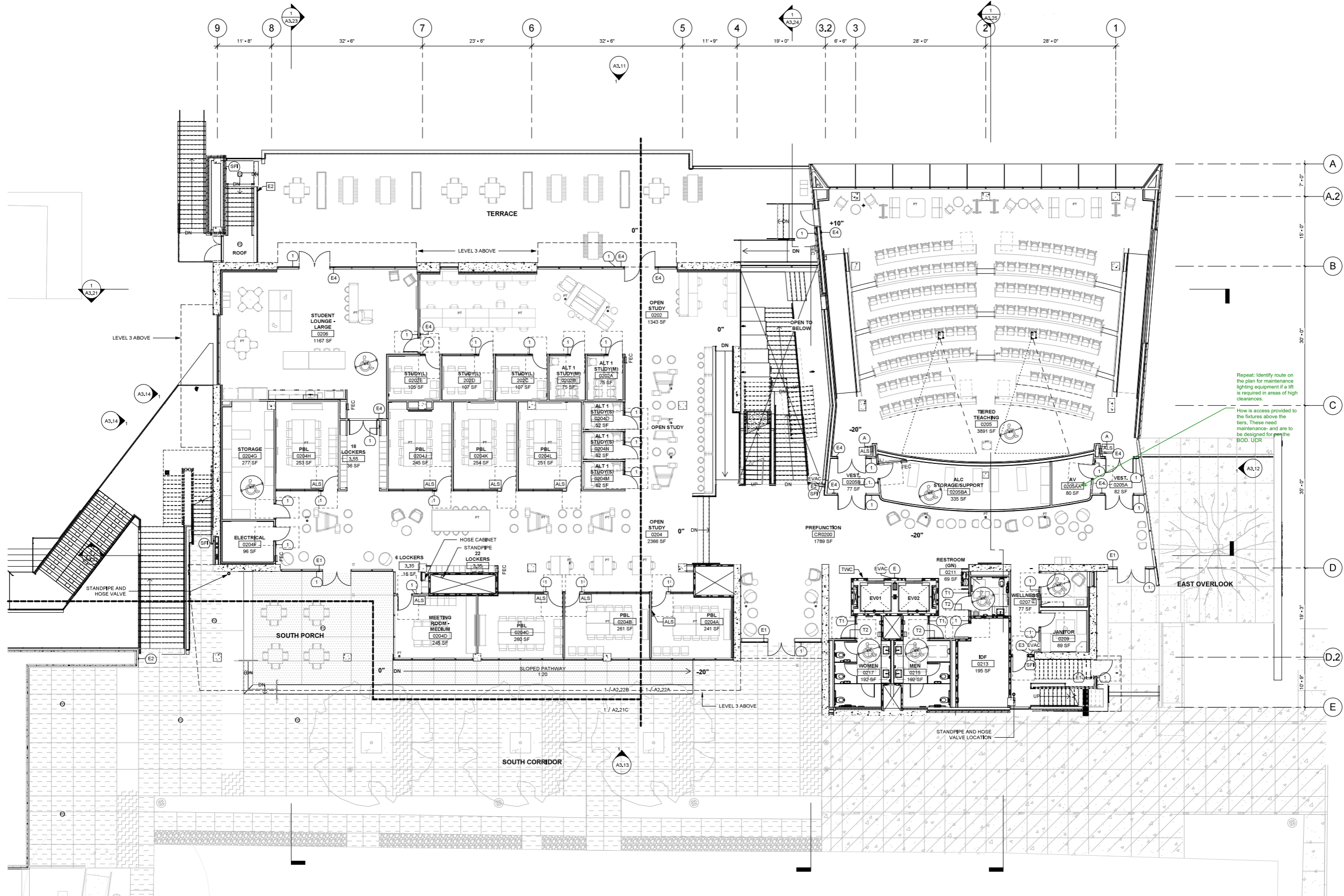
1 FLOOR PLAN LEVEL 02 1/8" = 1'-0"
